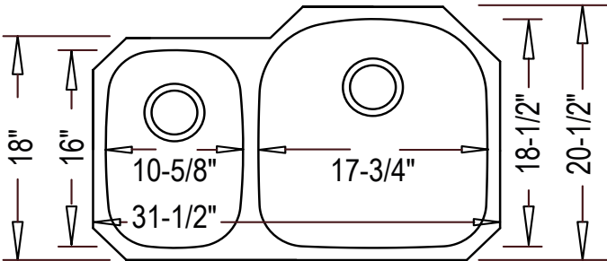
Product Diagram
