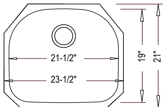
Product Diagram
