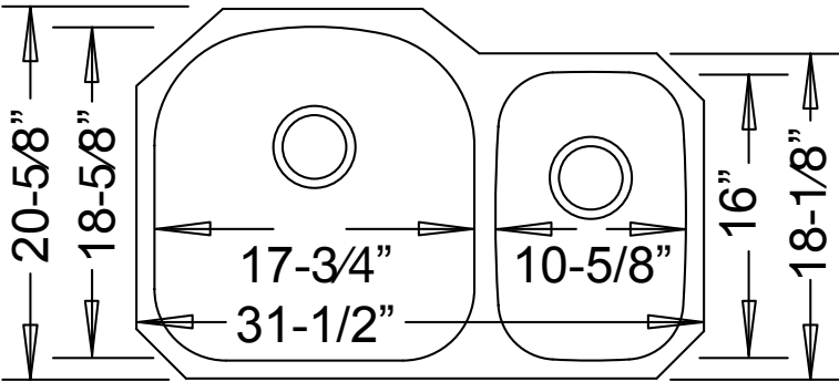
Product Diagram
