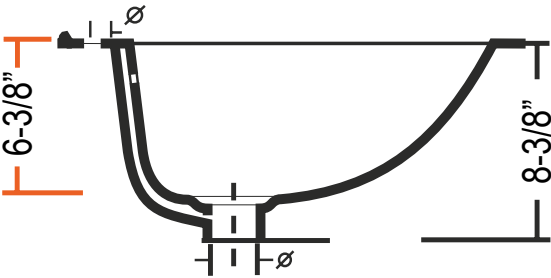
Product Diagram
