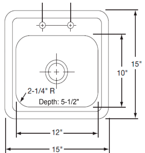
Product Diagram
